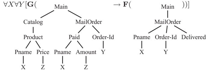
Fig. 5. Some Tree-LTL formulas.
