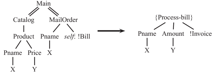
Fig. 3. Example of a relative query.
