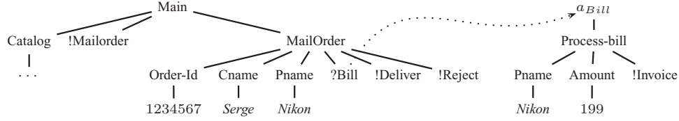
Fig. 4. An instance with an eval link.
